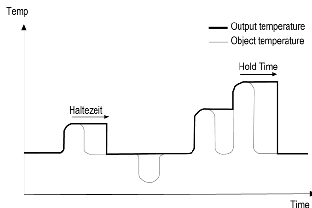
Figure 17: Peak Hold
