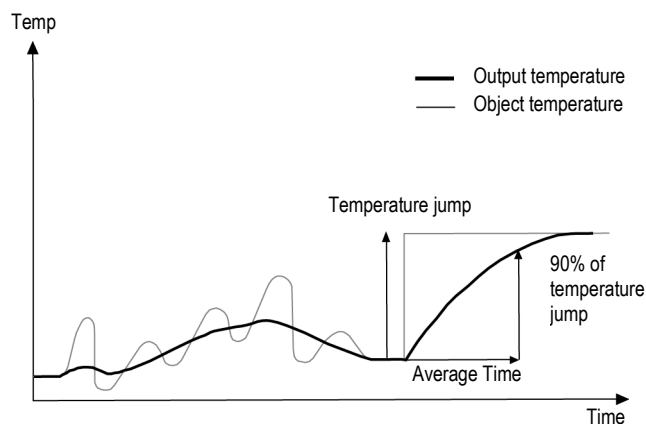
Figure 16: Averaging
