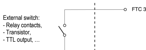
Figure 24: Wiring the FTC3 Input
