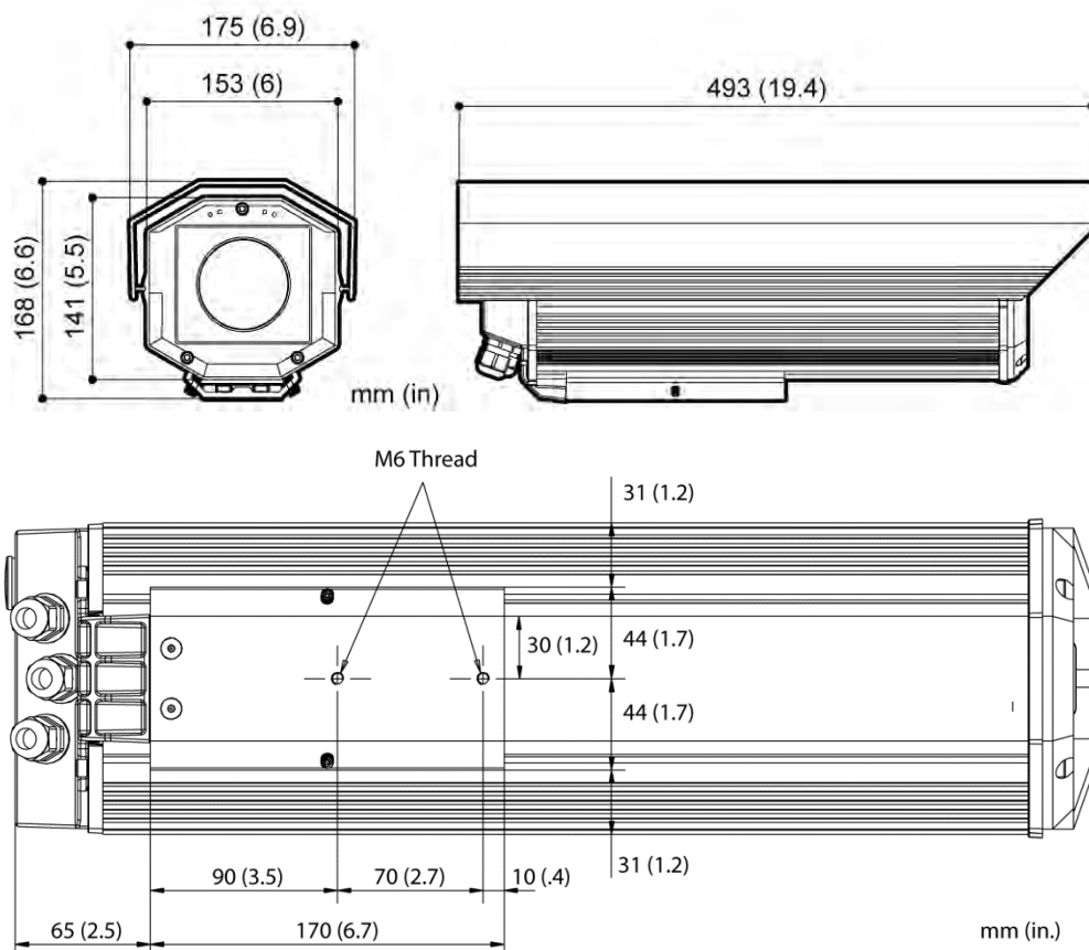
Figure 36: Dimensions and Footprint of Outdoor Enclosure (A-TV-ENC)
