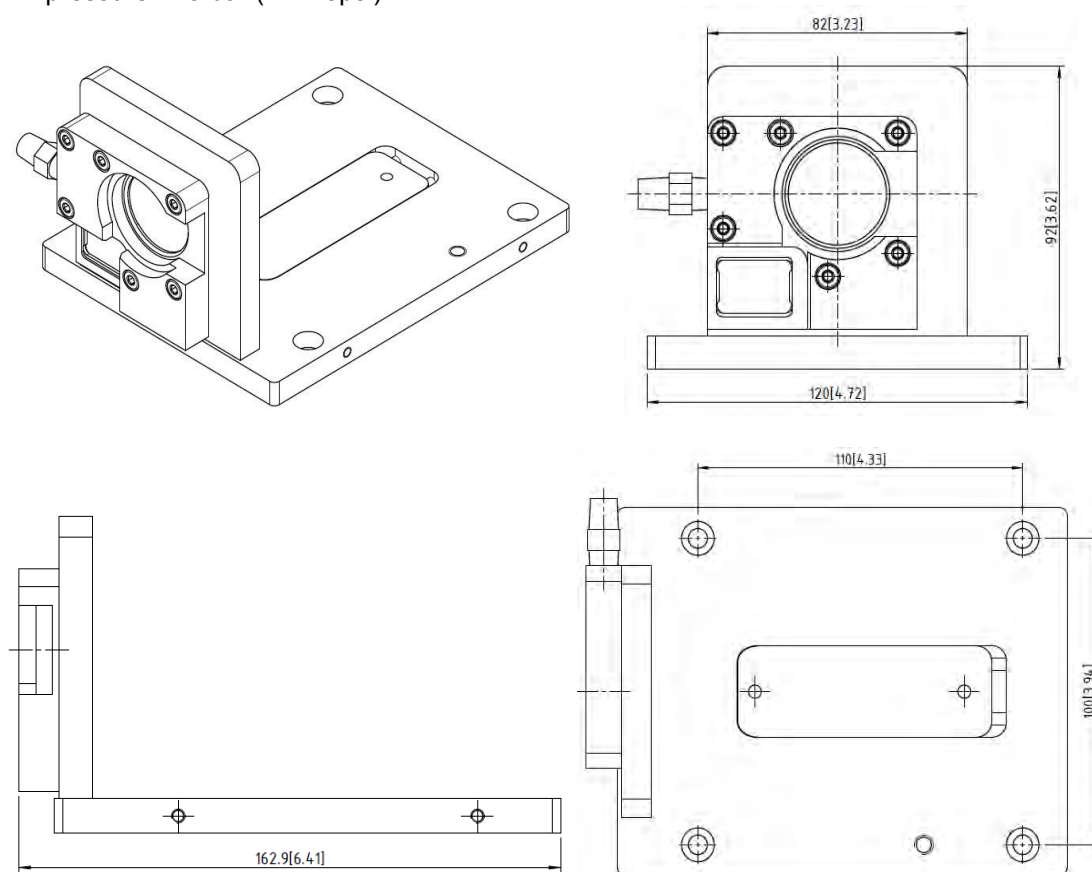
Figure 31: Air purge collar (A-TV-AP) without water cooling accessory
