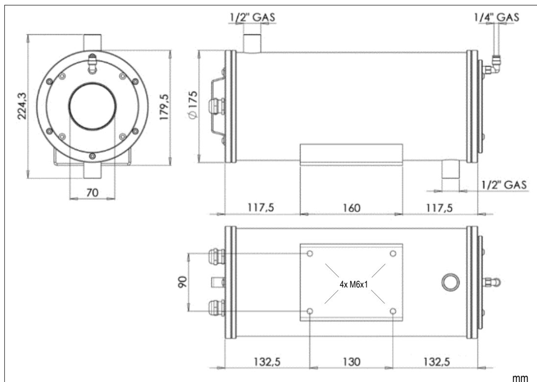
Figure 34: Dimensions of the Protective Enclosure (A-TV-WC)
