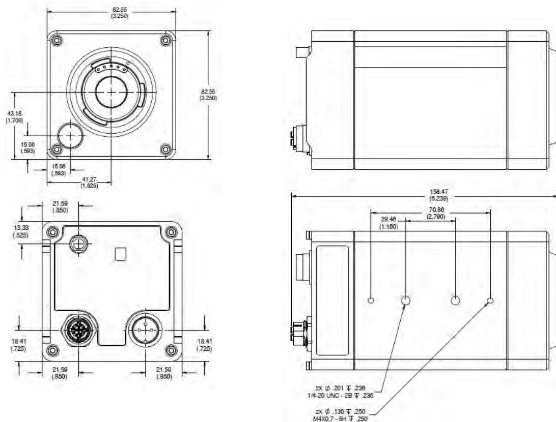
Figure 4: Front, Rear and Side View Dimensions of Standard ThermoView® Imager
